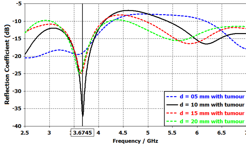
Figure 4.1 Simulated return loss with different values of d
