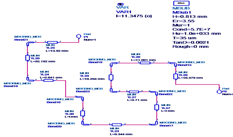
Figure A.1 ADS schematic for path 3
