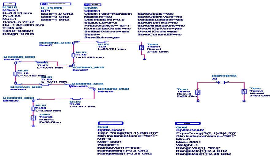
Figure A.2 ADS schematic to modify the length of path 3
