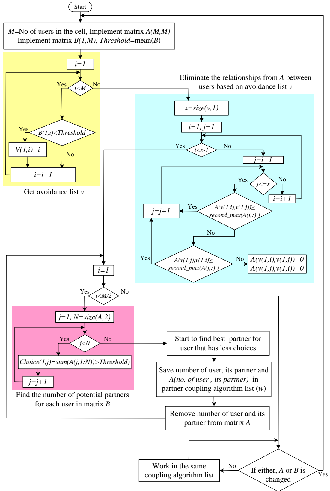
Figure 3.2 Flow chart for partner coupling algorithm
