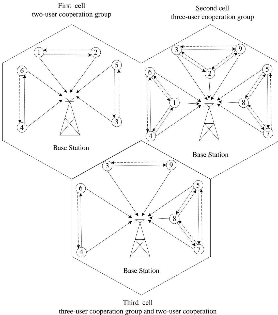
Figure 3.1 Partner coupling for user RS coded cooperation
