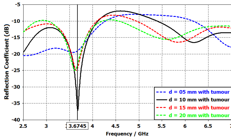
Figure 4.1 Simulated return loss with different values of d
